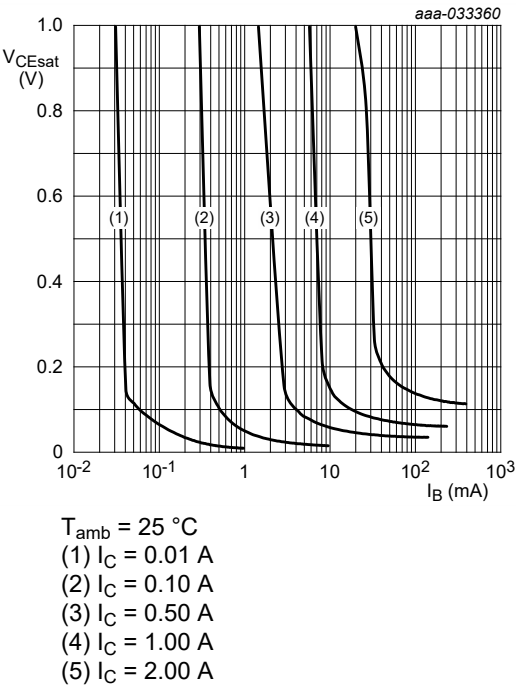
Fig. 8. Collector-emitter saturation region as a function of base current; typical values
