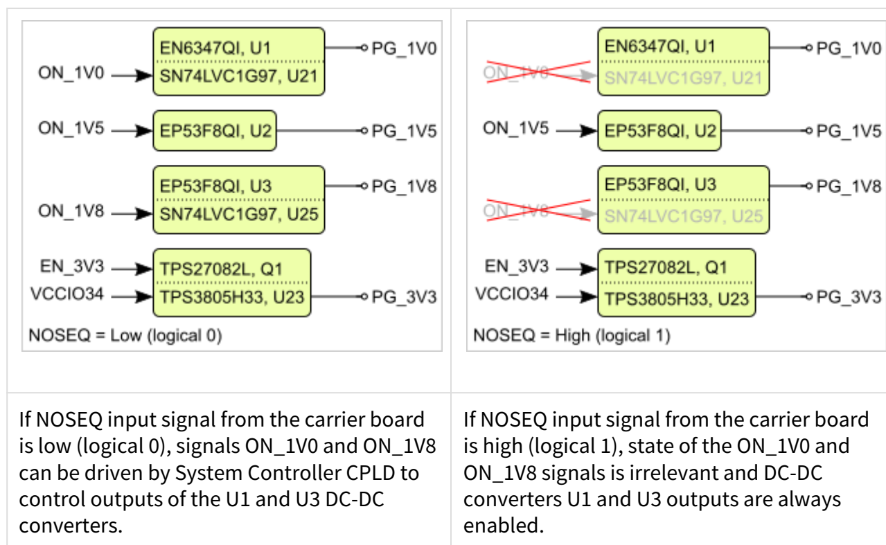
Figure 4: Power sequencing.
