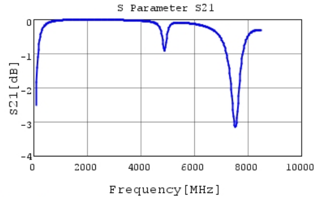
GCQ1555C1H180GB01 S21 DCOV, 25degC
