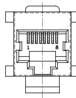
Front Panel Jack Only Clearance W/O Latch Feature
