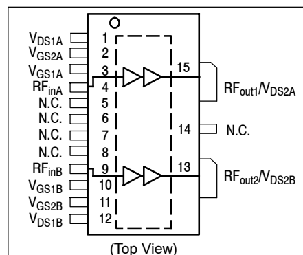
Figure 2. Pin Connections
