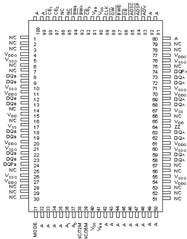
CY7C1382D (1M × 18)
