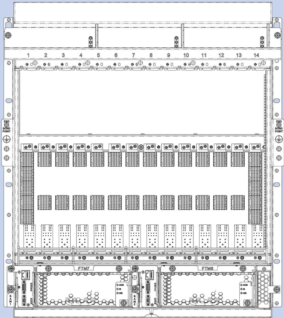
FRONT VIEW
