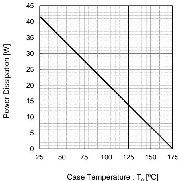
Fig.6 Power Dissipation
