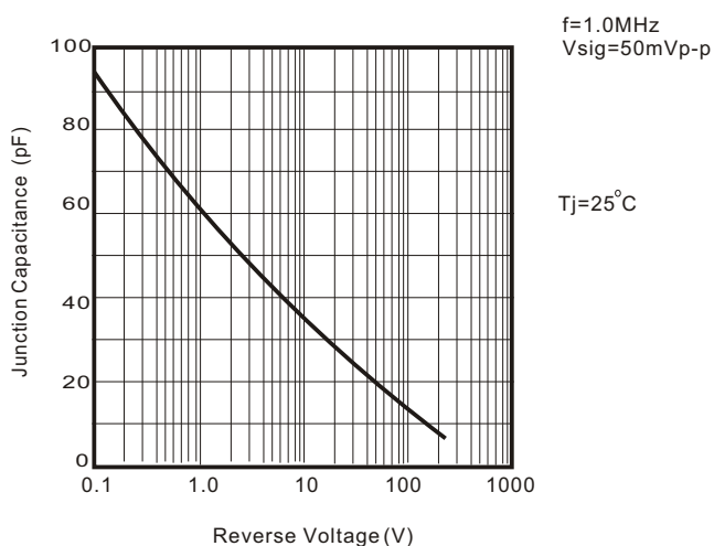
Fig. 3 - Junction Capacitance
