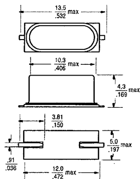
49SMLB package
