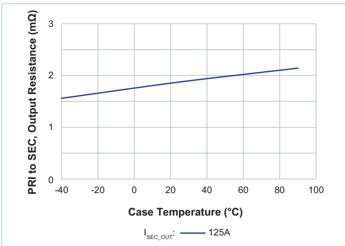
Figure 12 — R_{SEC} vs. temperature; Nominal V_{PRI\_DC} I_{SEC\_DC} = 100\text{A} at T_{CASE} = 90^{\circ}\text{C}
