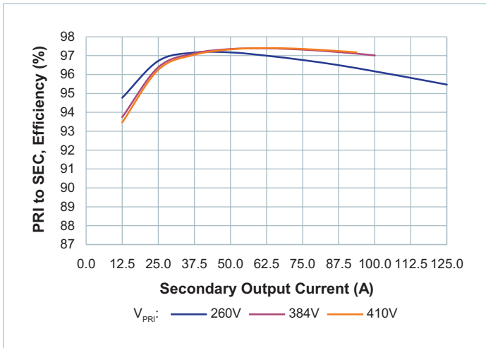
Figure 10 — Efficiency at T_{CASE} = 90^{\circ}\text{C}
