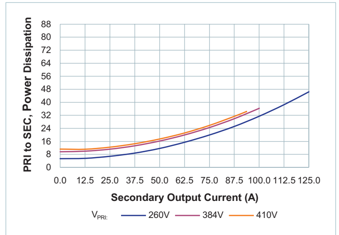
Figure 11 — Power dissipation at T_{CASE} = 90^{\circ}\text{C}
