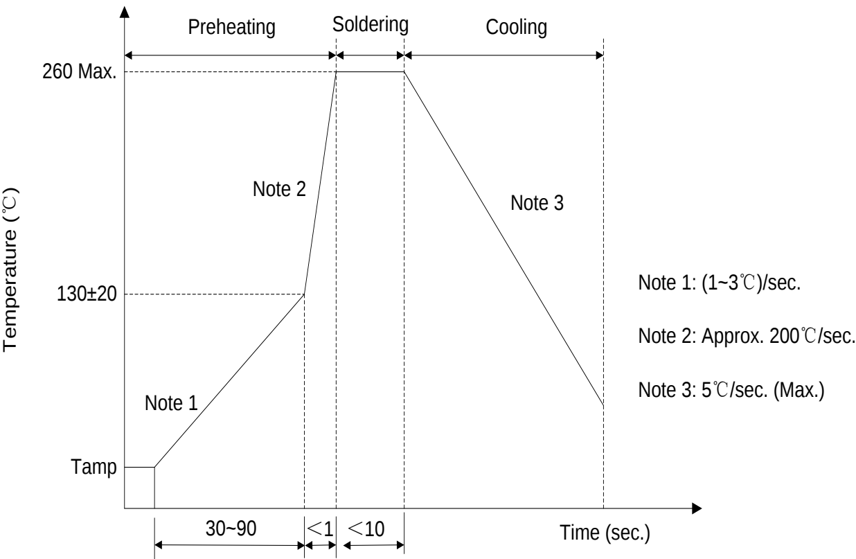
Recommendation Reworking Conditions with Soldering Iron
