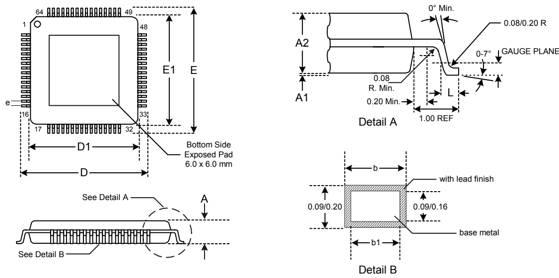
Figure 65. 64-Pin Thin Quad Flat Package (TQFP)
