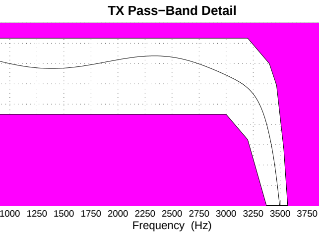
Figure 7. Transmit Path Frequency Response
