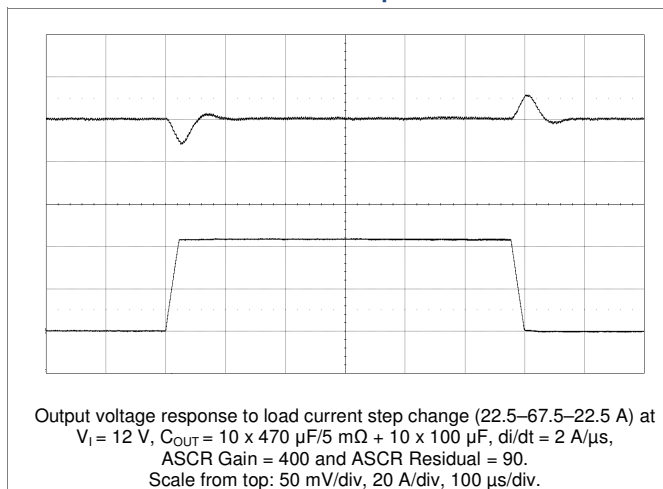
Transient Response
