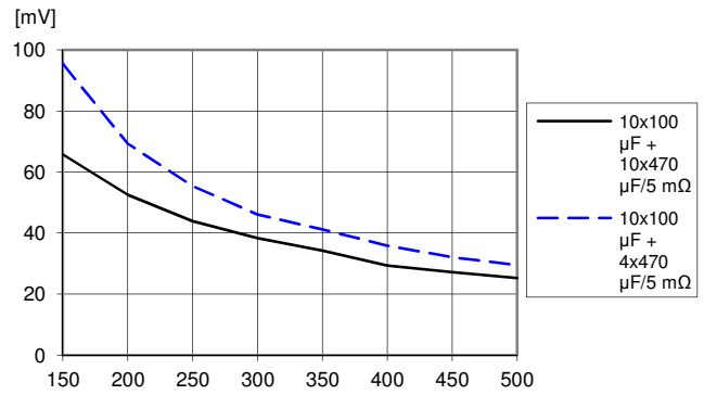
Load Transient vs. ASCR Gain and External Output Capacitance
