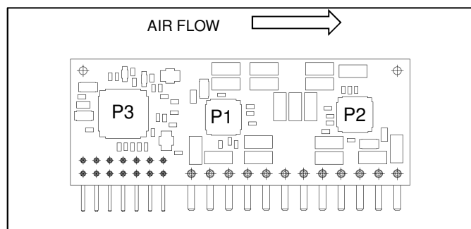
Temperature positions and air flow direction.
