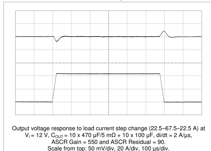
Transient Response
