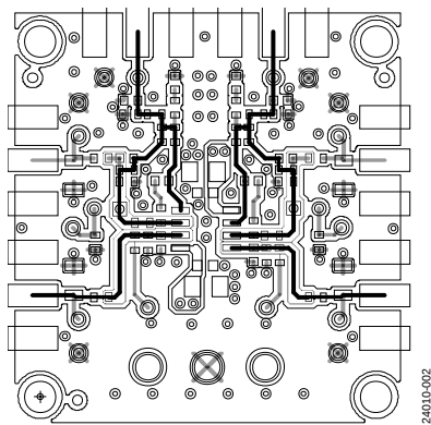
Figure 2. Default Connection
