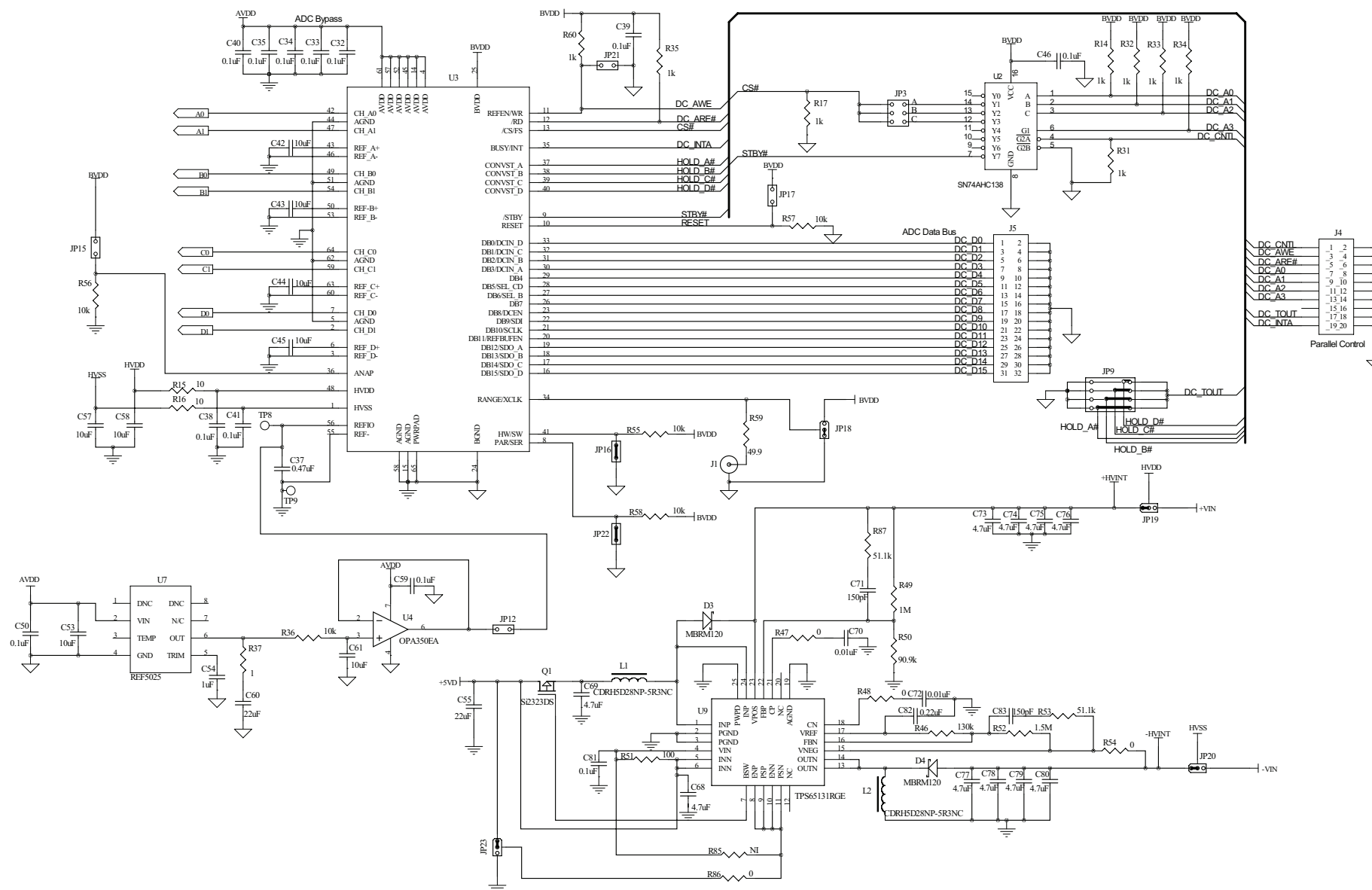
Figure 14. ADS85x8EVM: Schematic 2
