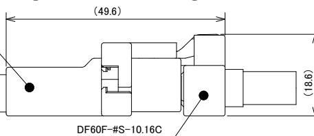
DF60F Finger Protection, Straight Socket
