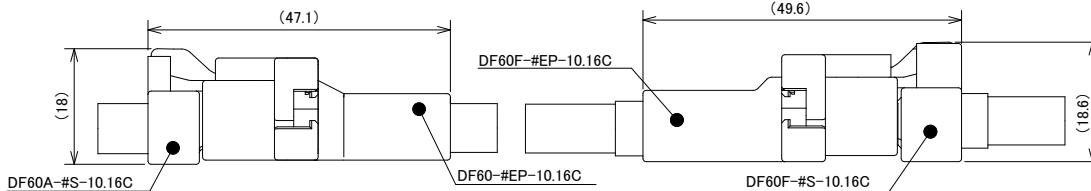
DF60FS Finger Protection, Right Angle Socket
