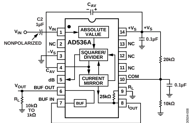
Figure 17. Single-Supply Connection
