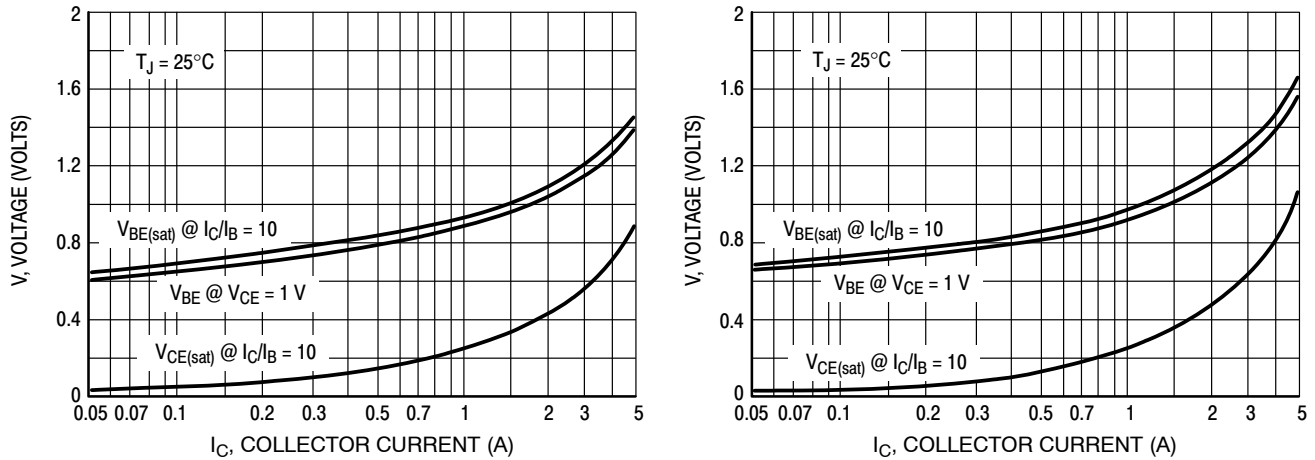
Figure 6. "On" Voltage
