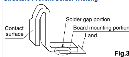
Structure Prevent Solder Wicking
