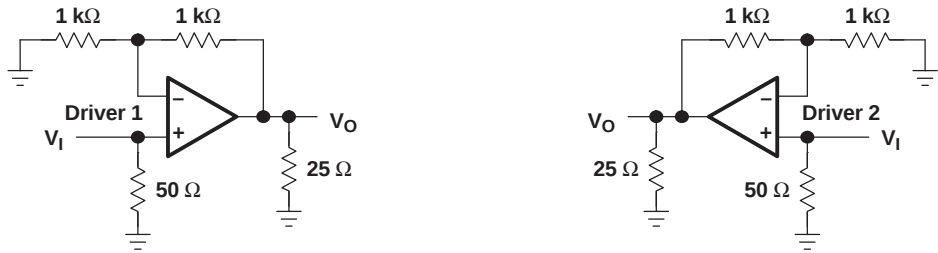
Figure 1. Input-to-Output Crosstalk Test Circuit
