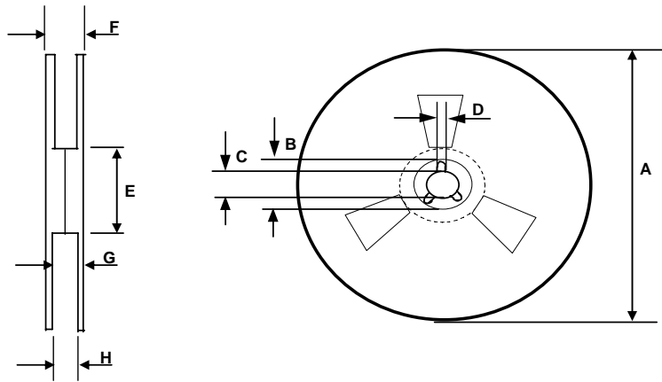
REEL DIMENSIONS FOR 20SOICW
