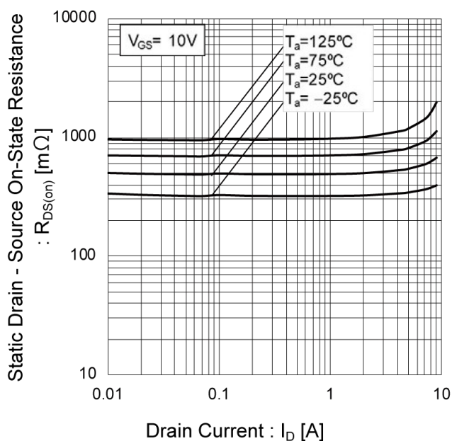
Fig.16 Static Drain - Source On - State Resistance vs. Drain Current(II)
