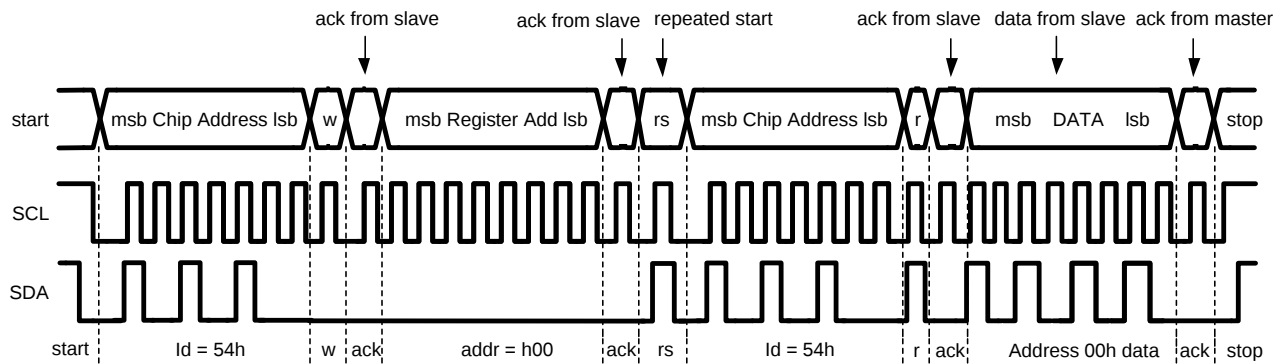
Figure 26. I²C Read Cycle
