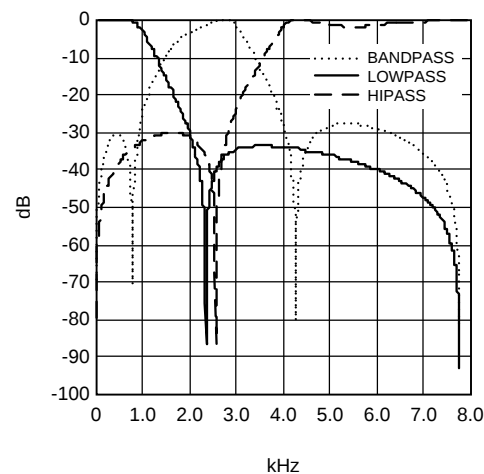
Figure 11. Lower frequency mode MODE_CTRL = 01 and SYNC_MODE = 1
