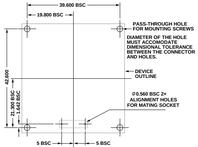
Figure 26. Mounting Example
