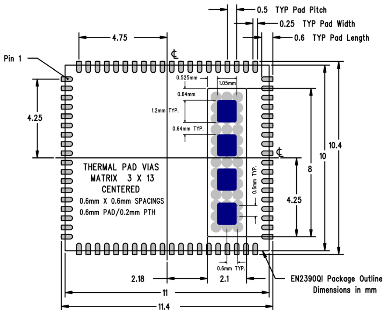
Figure 17: EN2390QI PCB Footprint (Top View)
