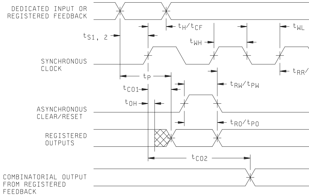
FIGURE 5. Switching waveforms.
