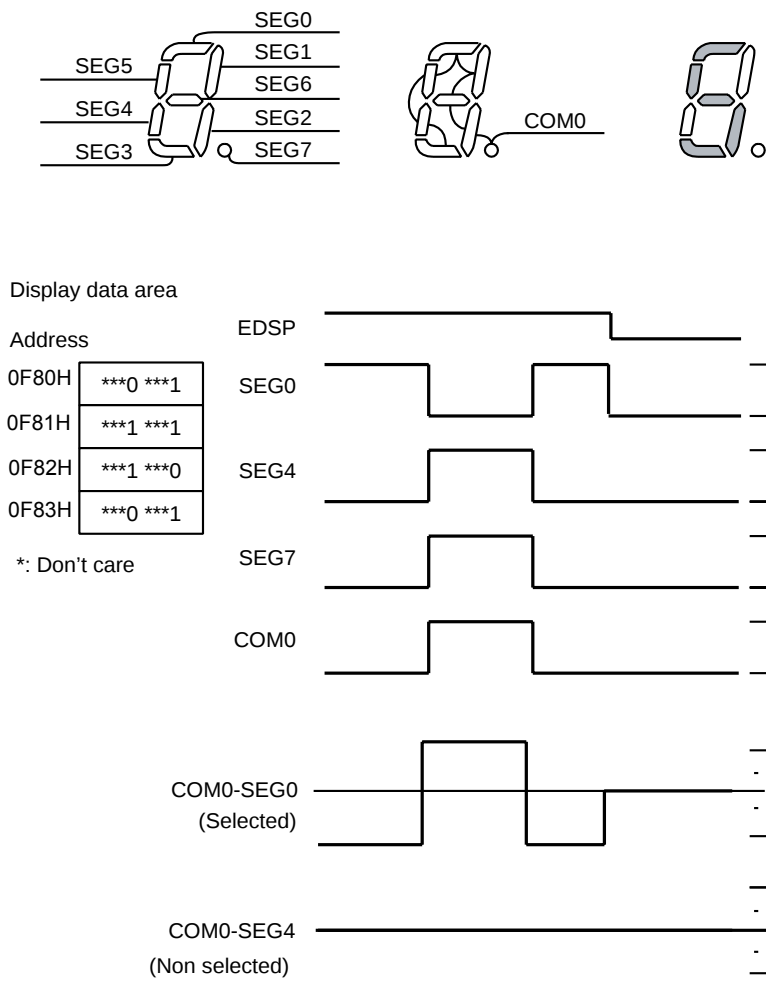
Figure 15-11 Static Drive
