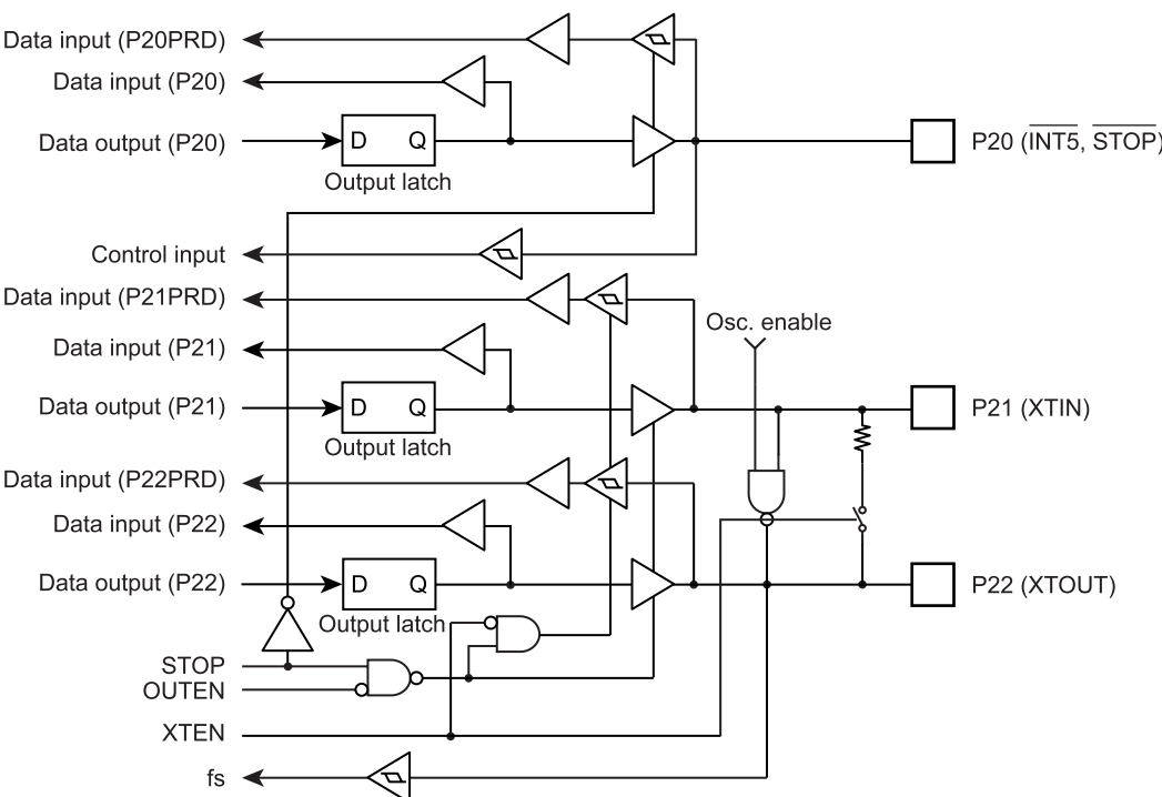
Figure 5-3 Port P2
