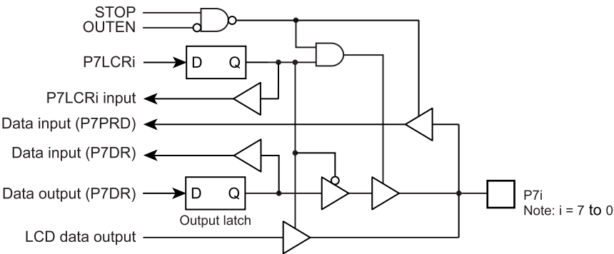
Figure 5-7 Port P7
