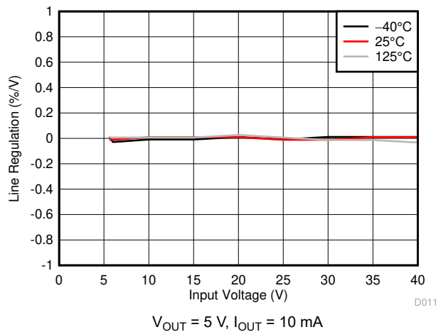
Figure 6-11. Line Regulation
