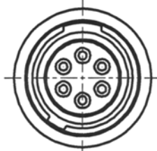
FRONT FACE VIEW SCE 6 WAY
