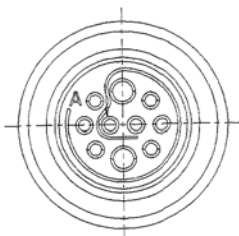
REAR FACE VIEW 10A WAY
