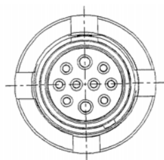
FRONT FACE VIEW 10A WAY
