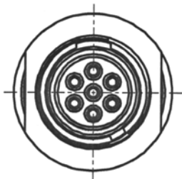
FRONT FACE VIEW SCE 7 WAY
