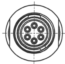
FRONT FACE VIEW SCE 6 WAY
