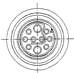
REAR FACE VIEW 10 WAY
