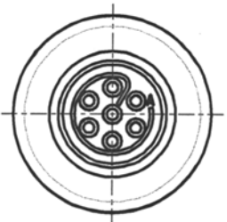
REAR FACE VIEW SCE 7 WAY
