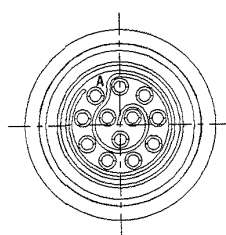
REAR FACE VIEW 12 WAY
