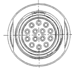
FRONT FACE VIEW 14 WAY
