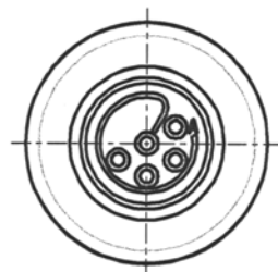
REAR FACE VIEW SCE 5 WAY
