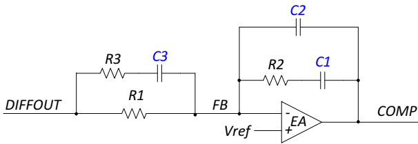
Figure 8. Error Amplifier
