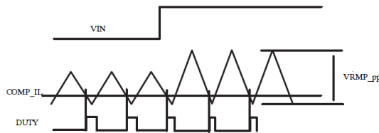
Figure 4. Ramp Feed Forward
