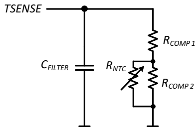
Figure 10. TSENSE Network
