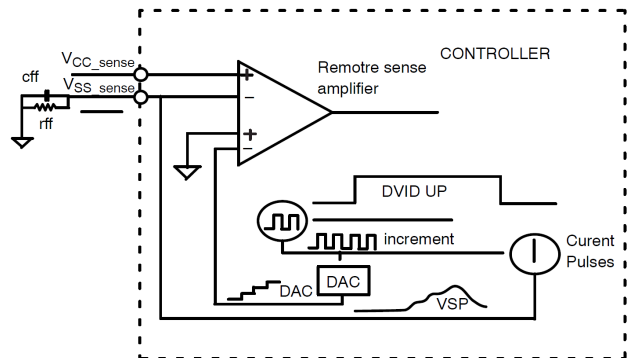
Figure 9. DAC Feed Forward
