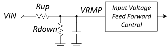
Figure 5. Ramp Feed Forward Circuit
