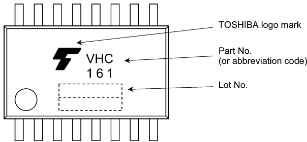
74VHC161FT
