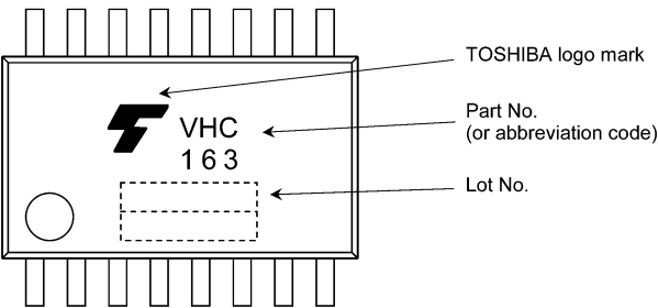
74VHC163FT
