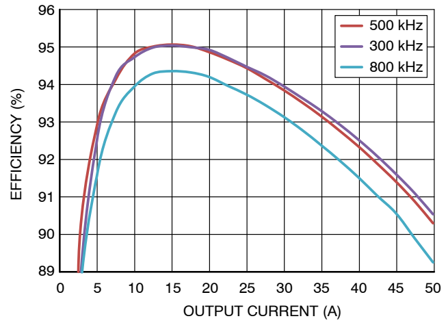
Figure 7. Efficiency – 12 V Input, 1.8 V Output
