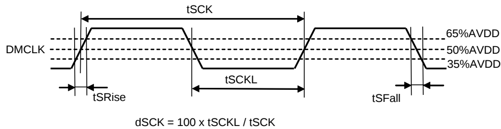
Figure 11. DMCLK Clock Timing
