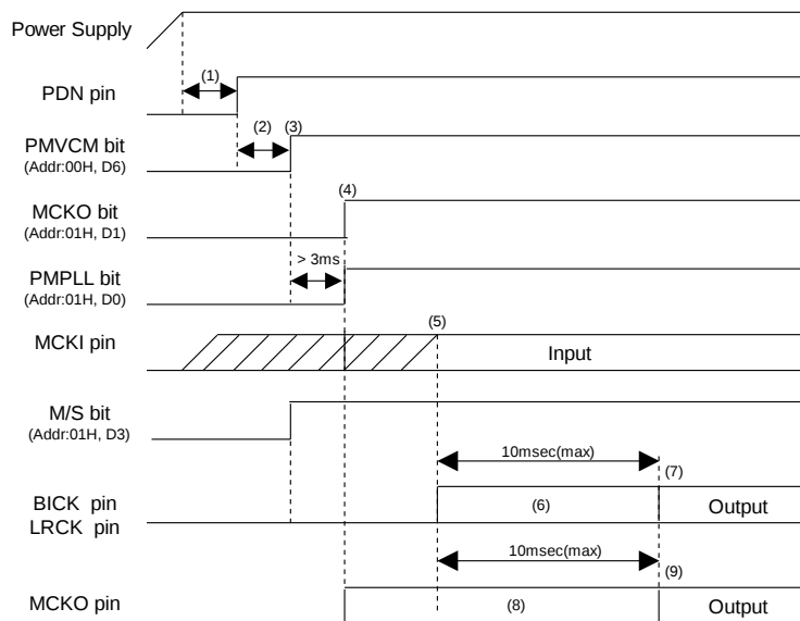
Figure 51. Clock Set Up Sequence (1)
