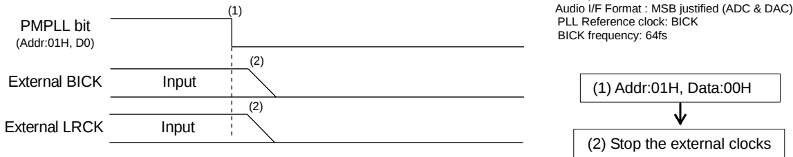
Figure 64. Clock Stopping Sequence (2)
