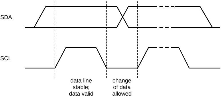
Figure 49. Bit Transfer (I 2 C Bus)
