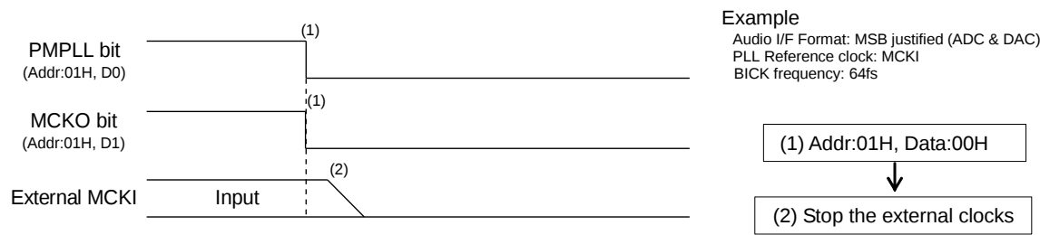
Figure 65. Clock Stopping Sequence (3)
