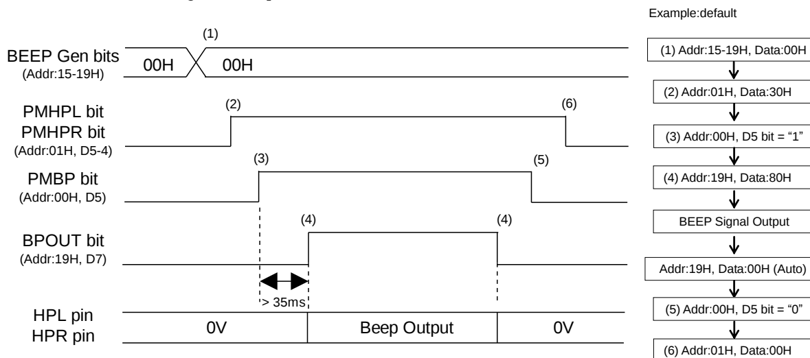
Figure 59. "BEEP Generator → Headphone-Amp" Output Sequence
