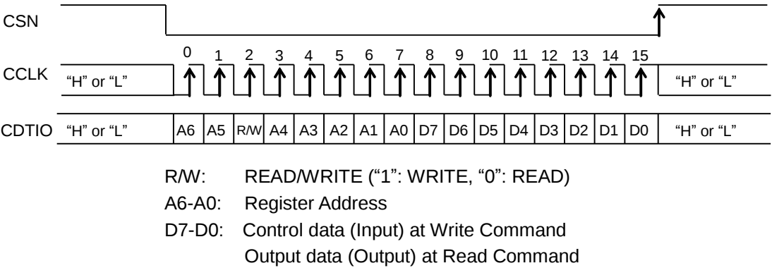
Figure 40. Serial Control I/F Timing
