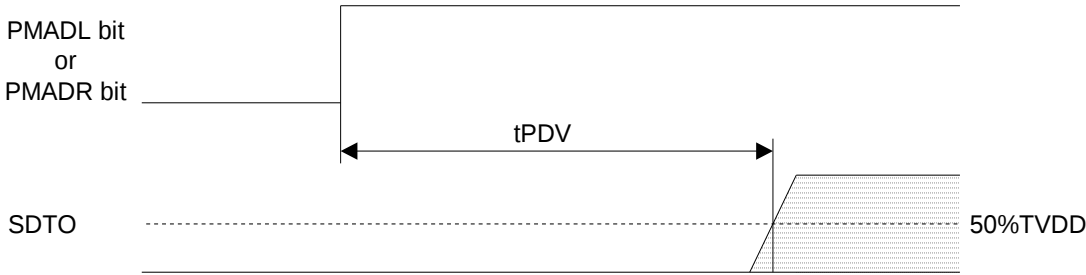
Figure 12. Power Down & Reset Timing 1
