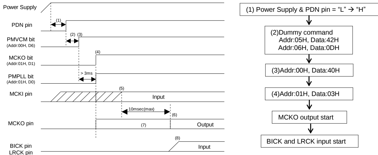
Figure 53. Clock Set Up Sequence (3)
