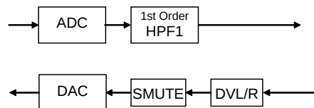
Figure 33. Path at Recording Mode 2 &amp; Playback Mode 2
