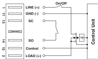
Block diagram
