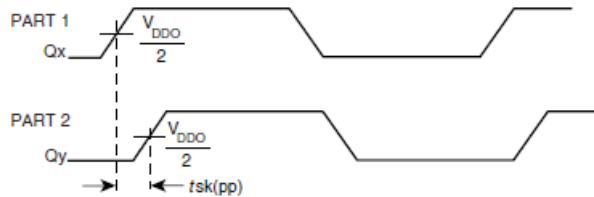
PART-TO-PART SKEW
