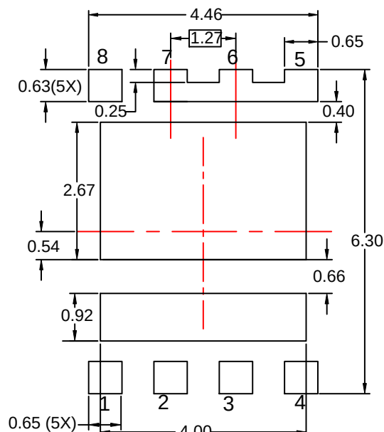
RECOMMENDED LAND PATTERN (OPTION 1 – FUSED LEADS 5,6,7)
