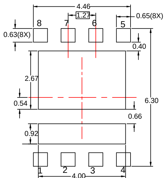
RECOMMENDED LAND PATTERN (OPTION 2 – ISOLATED LEADS)
