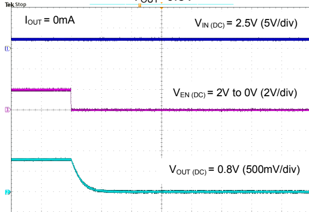
Enable Turn-Off Response V_{OUT}=0.8\text{V}
