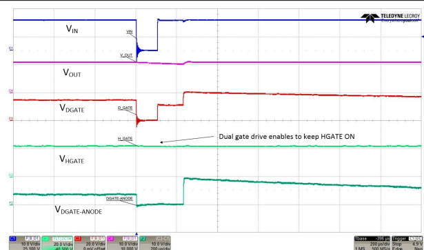
Figure 10-6. Input Micro-Short - LV124 E10 TC 2 100 \mu s with HGATE
