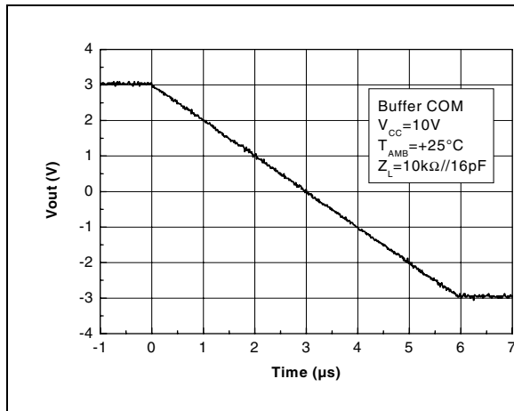
Figure 32. Large signal response - buffer COM
