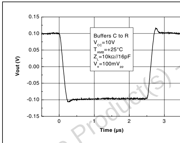
Figure 34. Small signal response - buffers C to R
