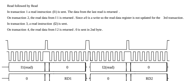
Figure 35. HPS SPI Read Timing (Read/Read)
