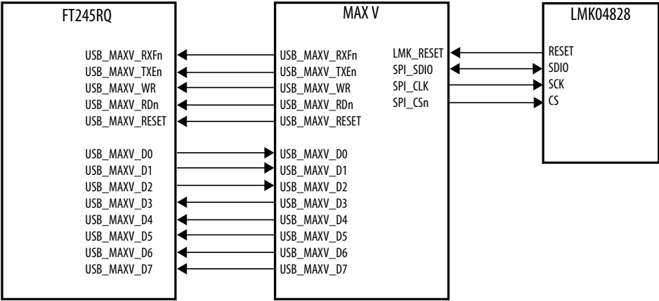
Figure 30. LMK04828 Controller
