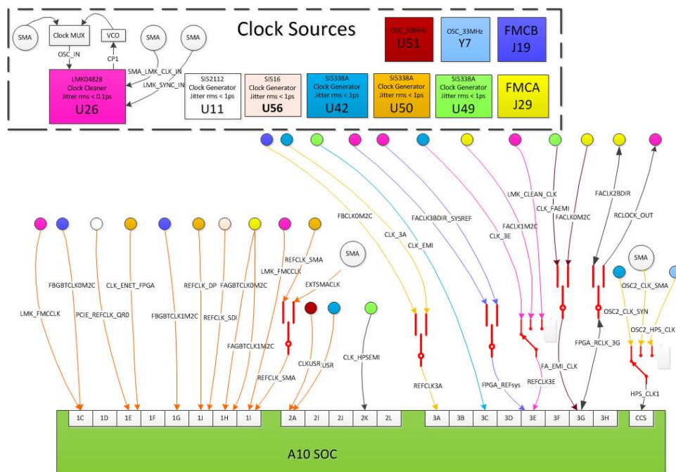
Figure 24. FPGA I/O Bank Clock Connection
