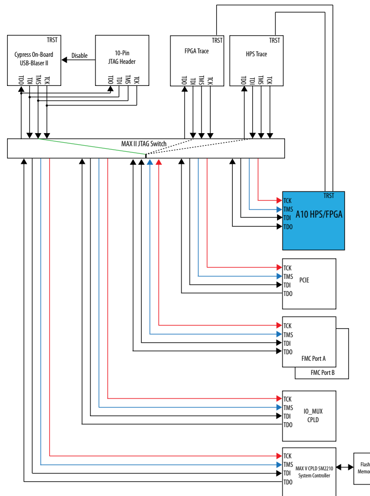
Figure 23. JTAG Chain
