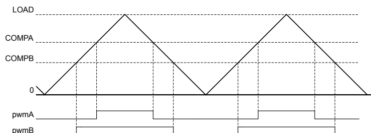
Figure 27-5. PWM Generation Example In Count-Up/Down Mode
