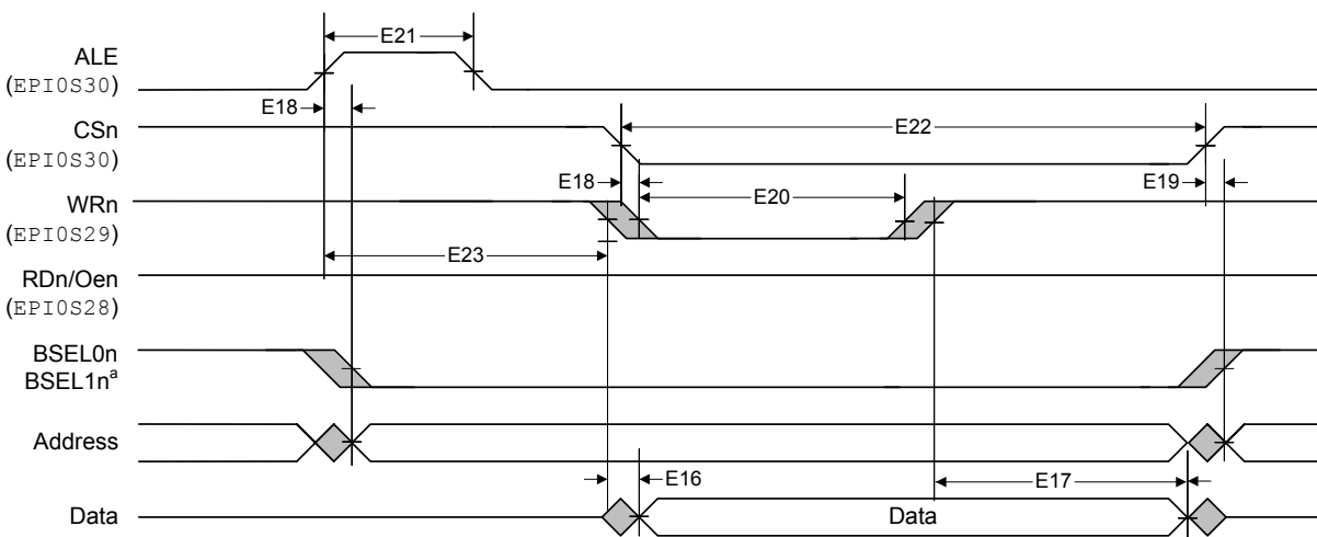
Figure 31-22. Host-Bus 8/16 Asynchronous Mode Write Timing
