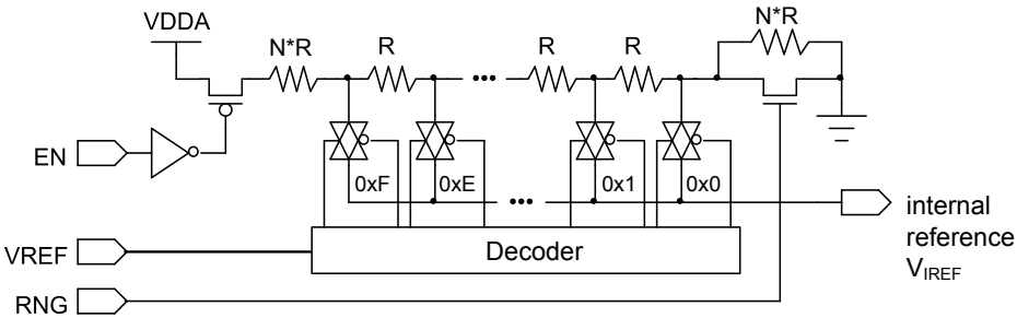
Figure 26-3. Comparator Internal Reference Structure
