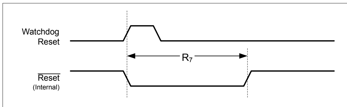
Figure 31-13. Watchdog Reset Timing
