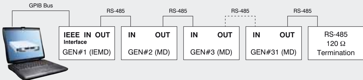
Multi-drop power supplies configuration
