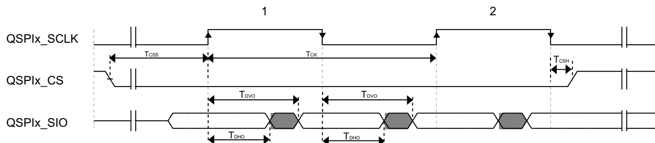
Figure 60. QuadSPI Output/Write Timing (DDR mode)
