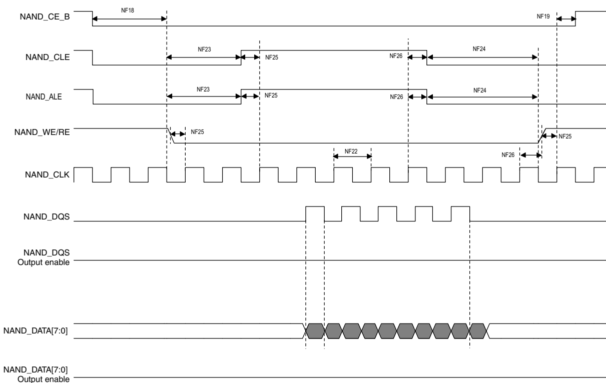
Figure 34. Source Synchronous Mode Data Read Timing Diagram
