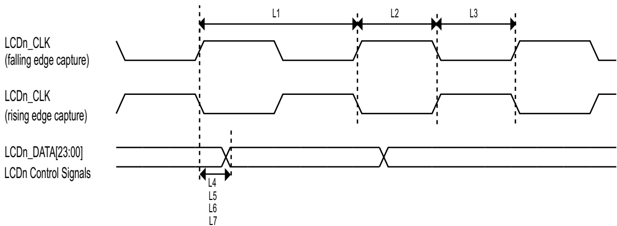
Figure 54. LCD Timing
