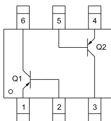
CMKT3906 (PNP/PNP) MARKING CODE: K06
