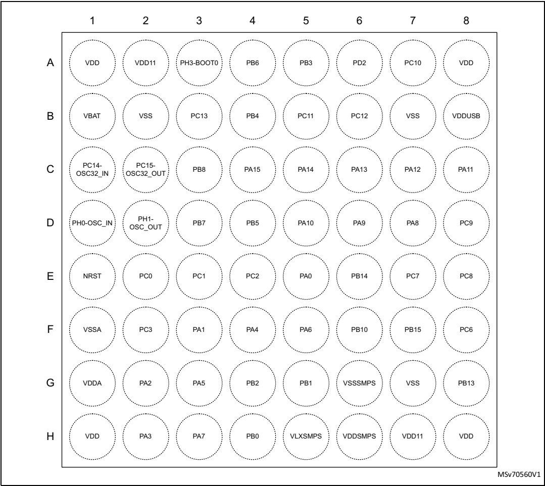
Figure 13. UFBGA64_SMPS ballout
