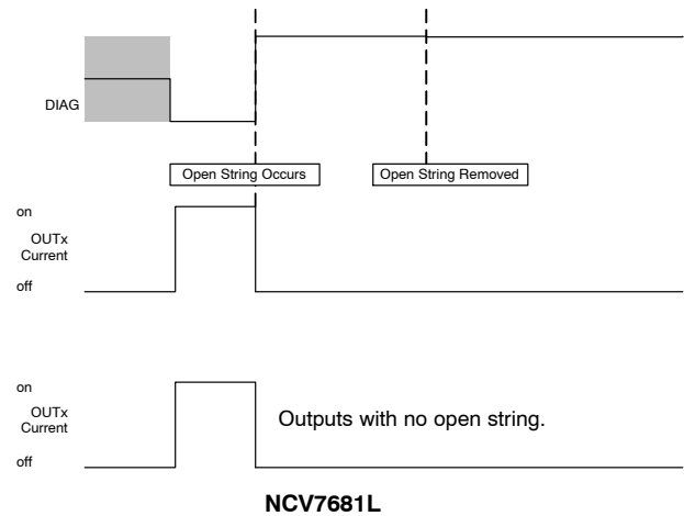
Figure 5. DIAG timing diagram WITH Open String Latch Active All outputs latch off.
