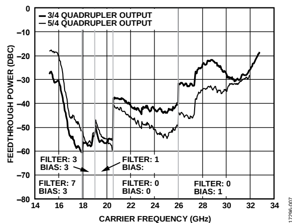
Figure 7. Aggregated Quadrupler Filter Performance, 3/4 Quadrupler Output and 5/4 Quadrupler Output
