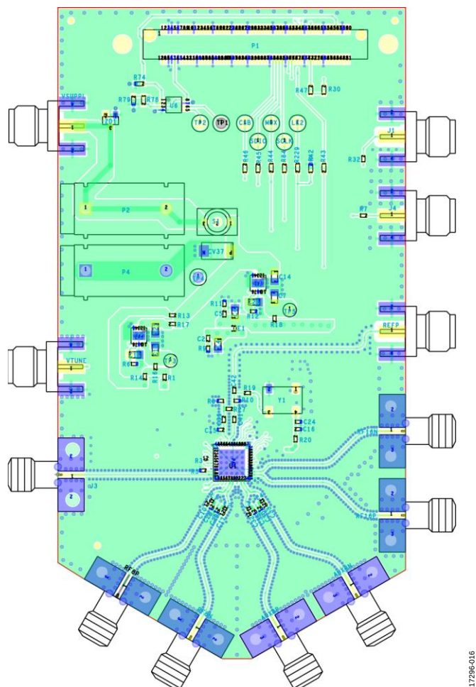
Figure 16. Evaluation Board Layer 1, Primary
