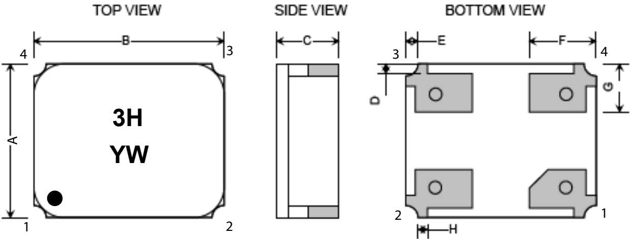
Dimensions in mm All pads have the same dimensions
