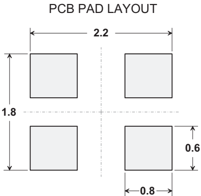
Dimensions in mm All pads have the same dimensions
