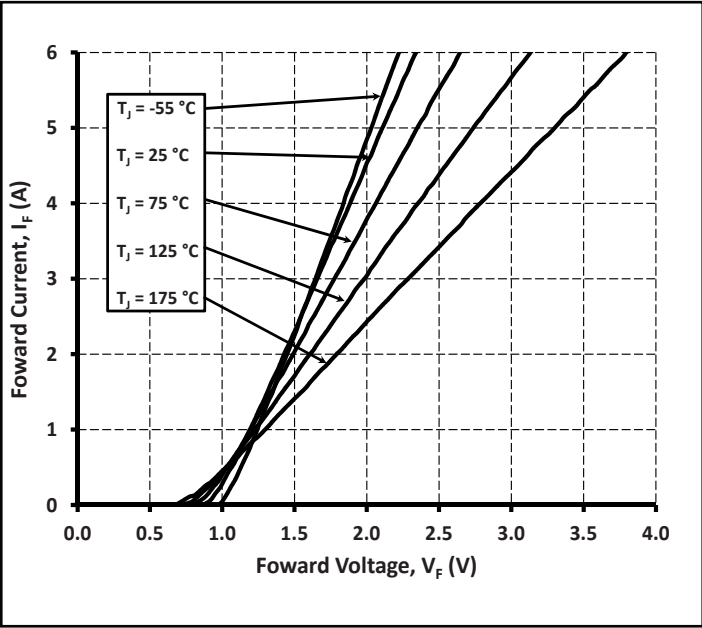
Figure 1 Forward Characteristics
