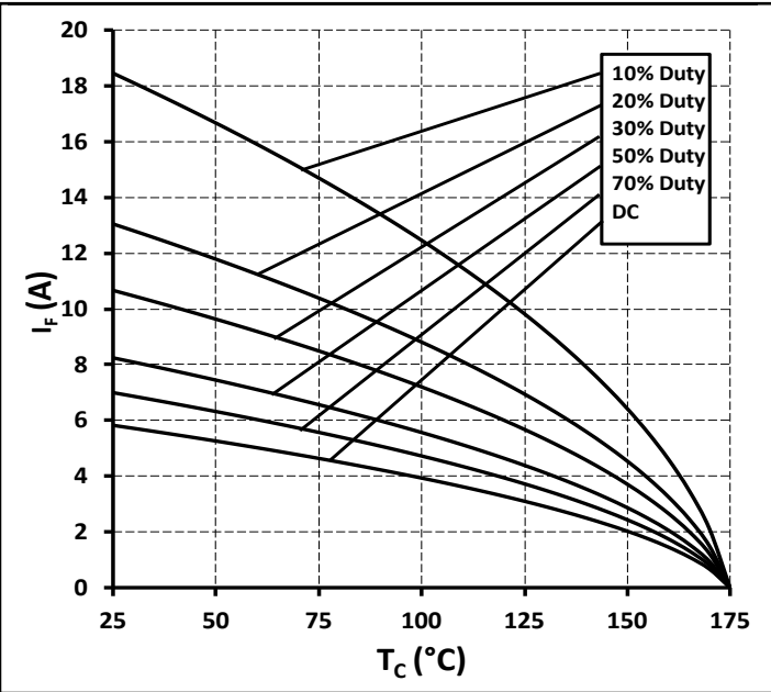
Figure 3 Current Derating
